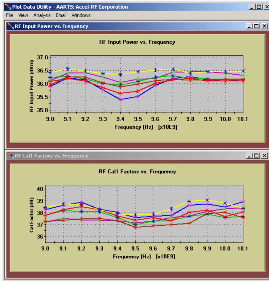
Figure 8: Calibration Plots
