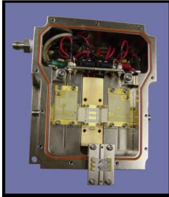
Figure 6: RF Fixture
