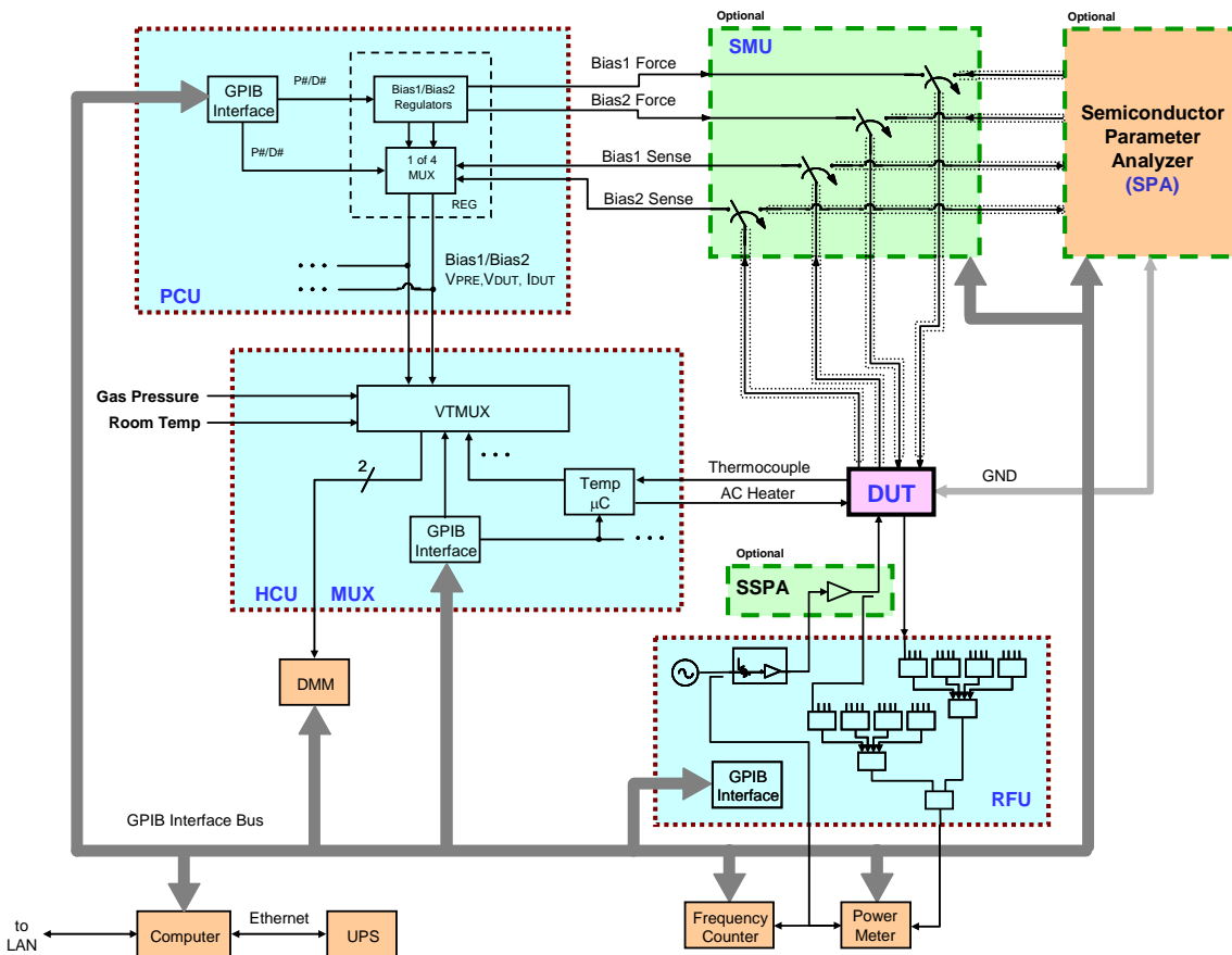
Figure 1: AARTS System Block Diagram
