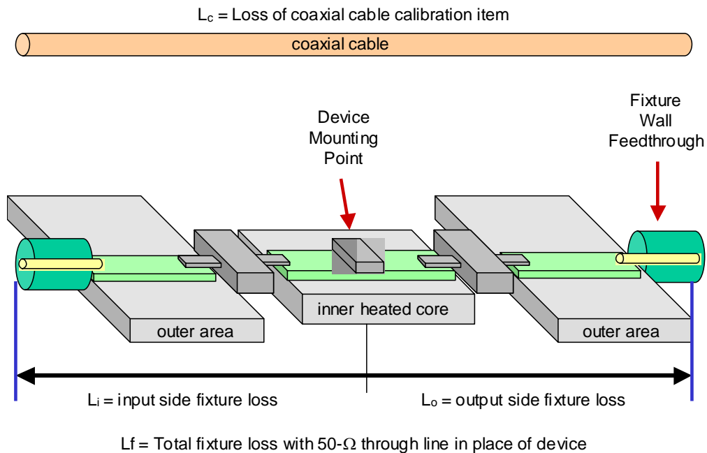
Figure 7: Fixture Losses
