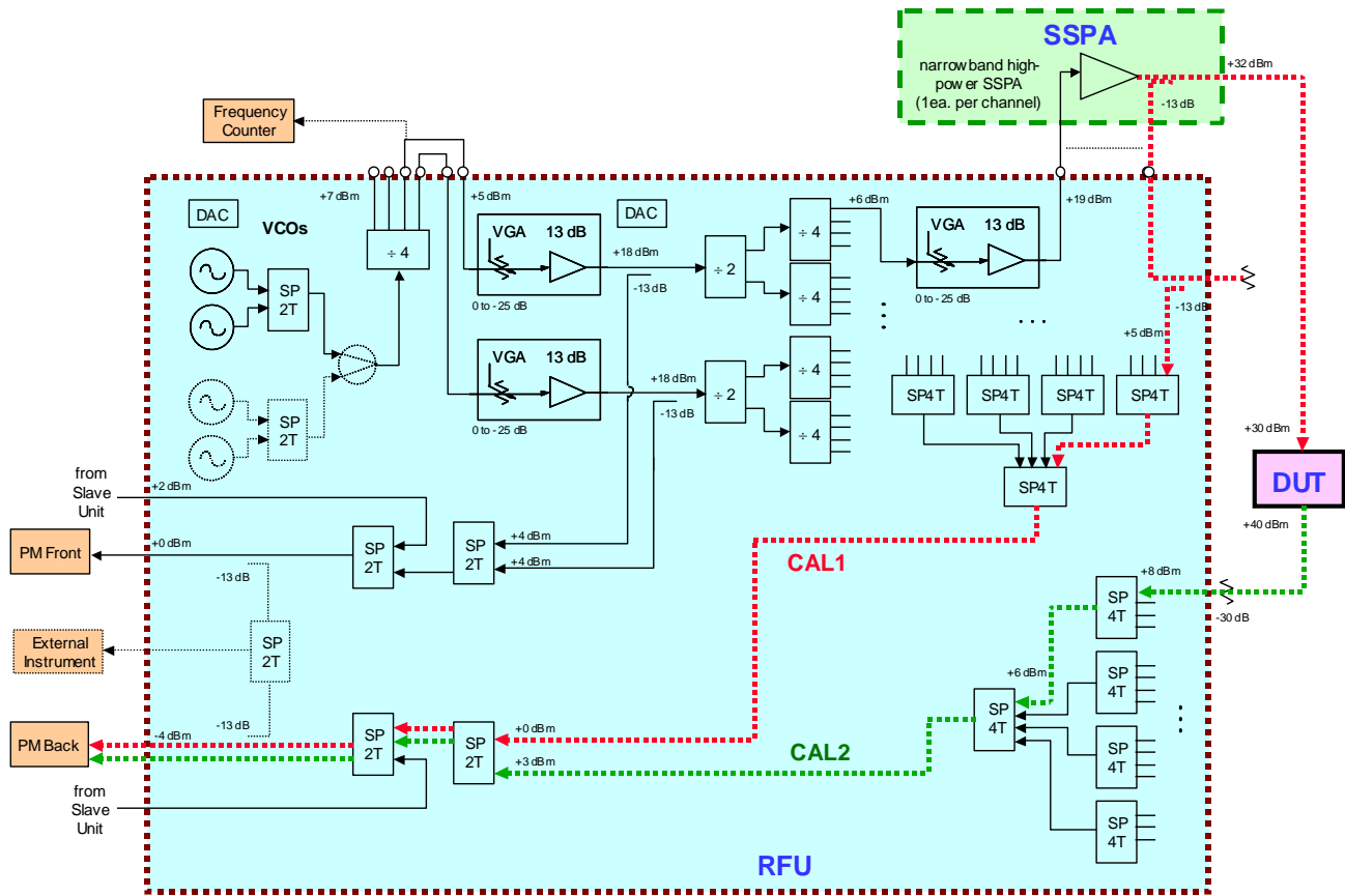
Figure 2: RFU Block Diagram
